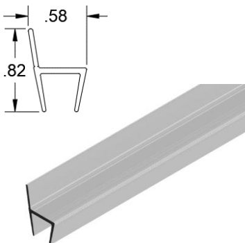
3/8" Wall Seal 98" M-P-SW38
