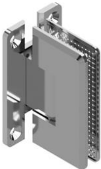
Beveled H Plate Glass-to-Wall Heavy Duty (110 lb./36" Width**) HI-HDBGTWFP Centerline or Adj. 0-5° Closing Beveled Edges Cutout Templates A, R
