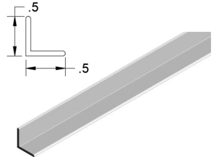
L-Angle Striker 1/2x1/2 w/Tape 98" M-P-1/2x1/2-98
