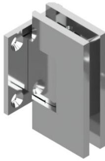
Adjustable Short Plate Glass-to-Wall Deluxe (80 lb./28" W max*) HI-DGTWADJSP Self-Centering 0° Return with Adjustment Up to 30° In or Out Squared Edges Cutout Template K
