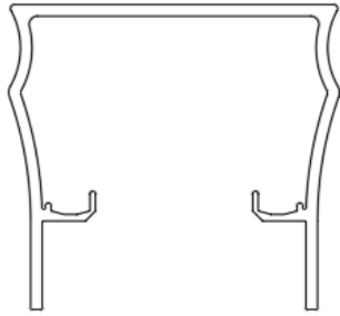
B. E-FSWJ - Framed slider wall jamb
