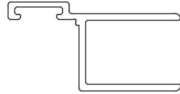
H. M-FDM - Black magnetic strip
