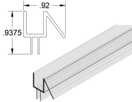
3/8" Glass Door Sweep 98" M-P-38DS
