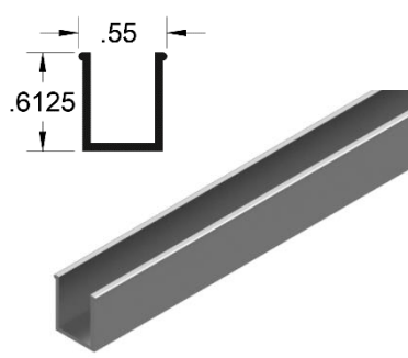
3/8" Header Snap Insert 6ft
