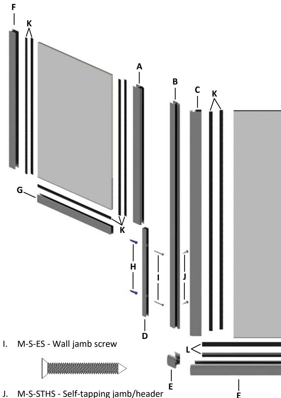
E. E-HEF - Header/Base of assembly
