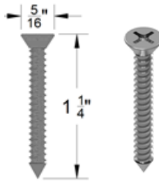
Enclosure Extrusion Screw M-S-ES
