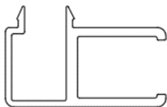
E. V-V-14 – 1/4" vertical vinyl
