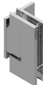
Offset Plate Glass-to-Wall Heavy Duty (110 lb./36" Width**) HI-HDGTWOP Centerline Closing Squared Edges Cutout Templates B, M
