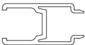
B. E-APR – Adjustable post receiver
