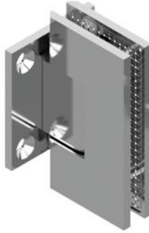
Adjustable Short Plate Glass-to-Wall Heavy Duty (110 lb./36" Width**) HI-HDGTWADJSP Self-Centering 0° Return with Adjustment Up to 30° In or Out Squared Edges Cutout Templates A, R
