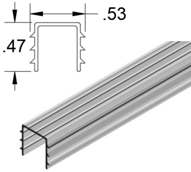
3/8" Euro Header Glazing Vinyl V-38-B
