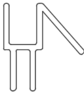
F. M-SFLSP - Semi-frameless strike plate with rubber mounting bladder
