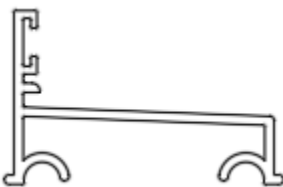
D. V-14BTGS - 1/4" Semi-frameless slider bottom track insert strip
