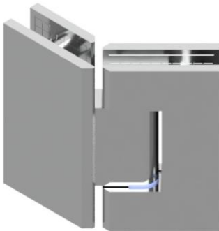
135° Glass-to-Glass Deluxe (80 lb./28" W max*) HI-DGTG135 Adjustable 0-5° Closing Squared Edges Cutout Template D
