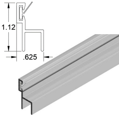
3/8" Poly Strike 180 Degree (removable fin) 98" M-P-38180SJ
