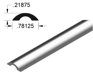
Half Moon Threshold
