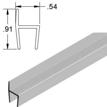
3/8" Strike Hard-H 98" M-P-38HJ
