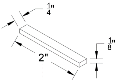
1/8" Setting Block M-SB-18
