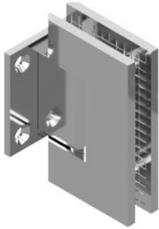
Short Plate Glass-to-Wall Heavy Duty (110 lb./36" Width**) HI-HDGTWSP Centerline or Adj. 0-5° Closing Squared Edges Cutout Templates A, R
